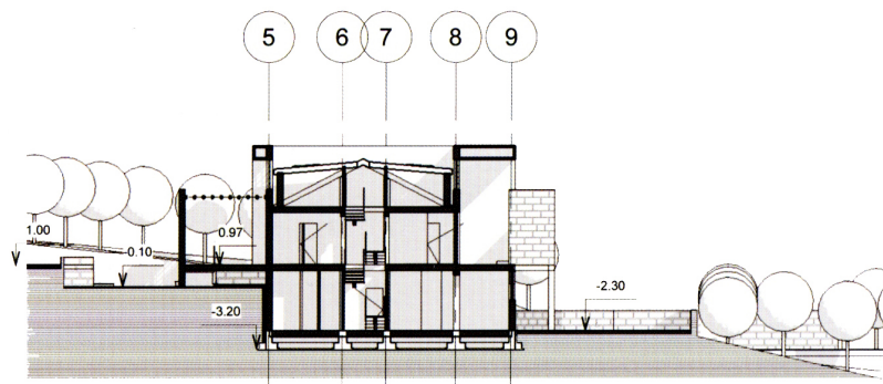
14 Cross profile A101 1 : 200
